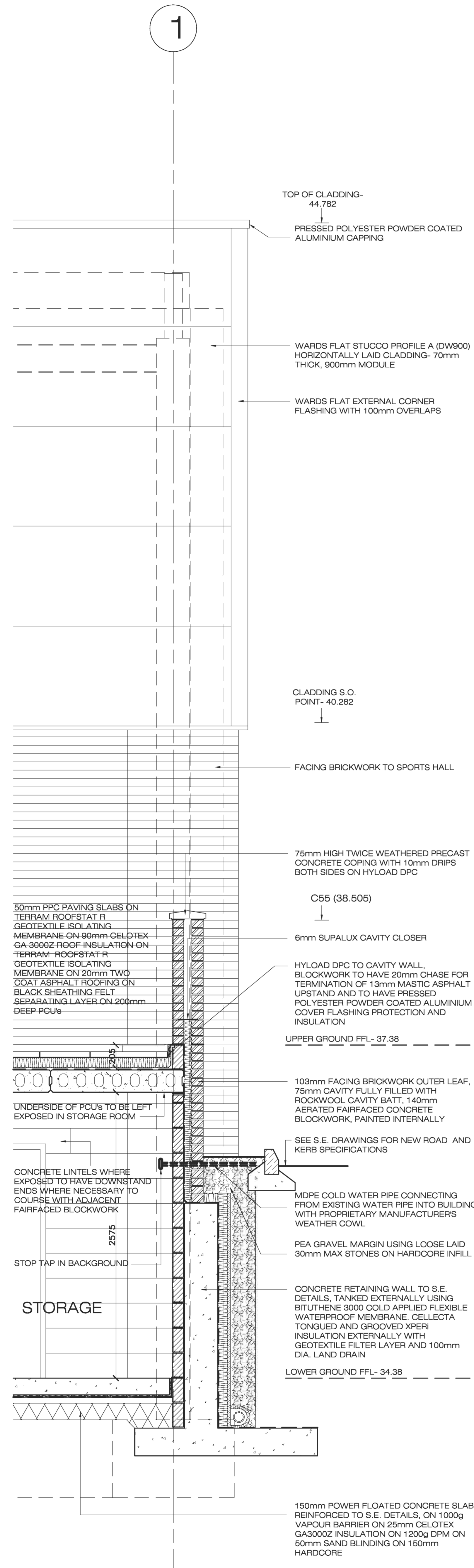
LINK SECTION ALONG GRID LINE 1
